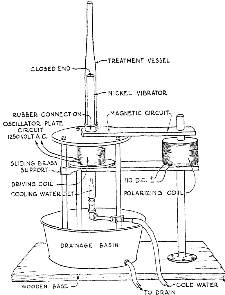
FIG. 4. Magnetostriction sound generator (from L. A. Chambers and E. W. Flösdorf); reproduced by permission.
