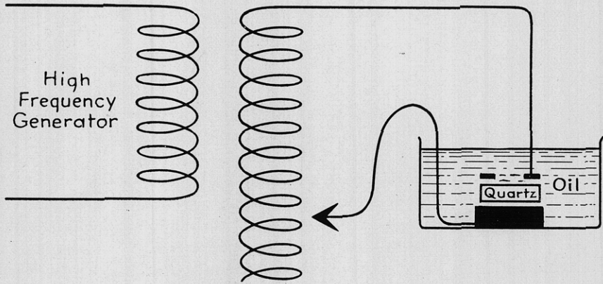
FIG. 1. Piezoelectric sound generator
