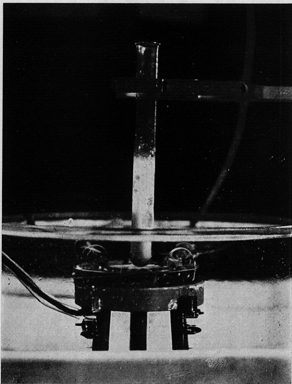
FIG. 3. Quartz oscillator and electrode system of a piezoelectric sound generator in an oil bath as used for emulsification (from K. Sollner).
